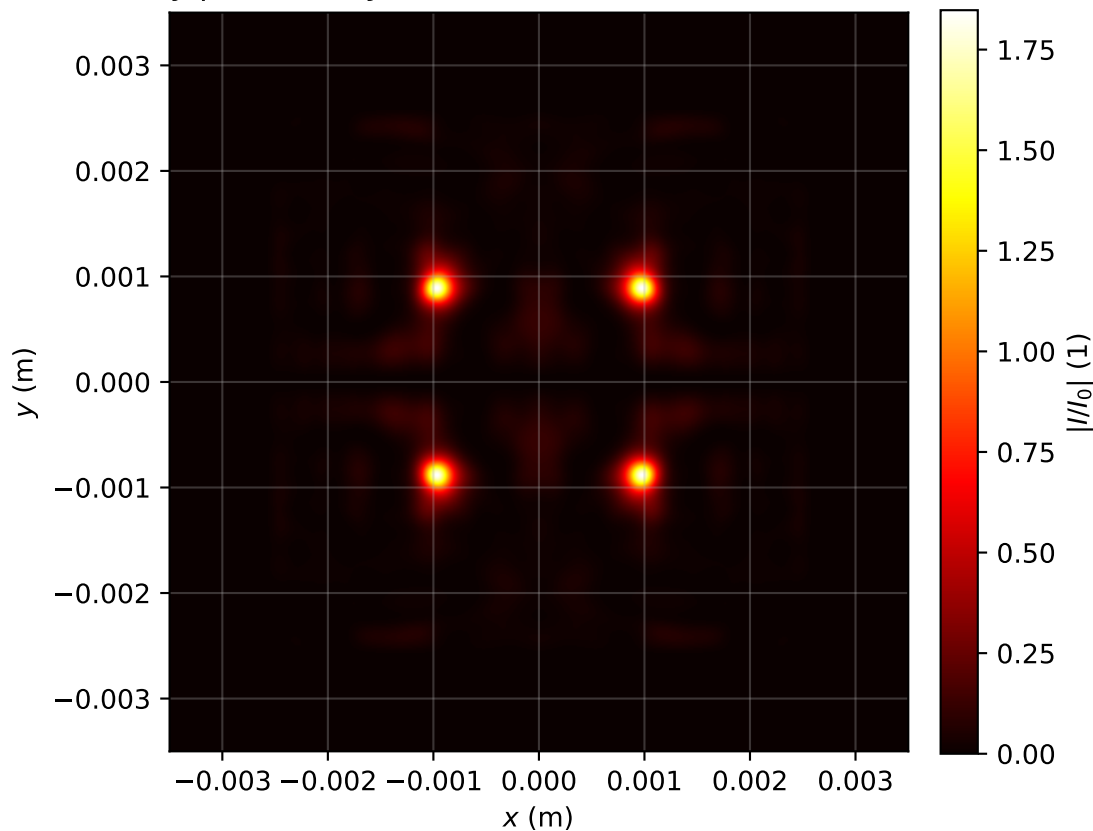
Intensity profile I(x, y, z = 3.025)/I_0 , P_{in}=9.0P_{cr} , artificial time
